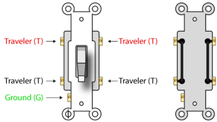
4 Way Switch Or Crossover How To Wire A Light
